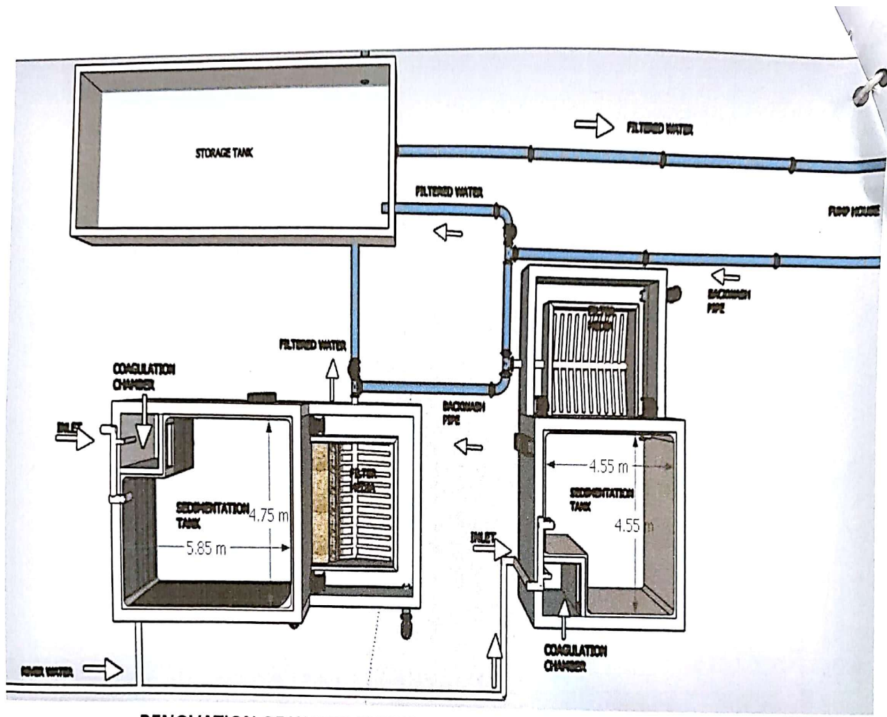
RENOVATION OF WATER SUPPLY SYSTEM AT KLHEP, PUMP HOUSE, LENGERY COLONY
